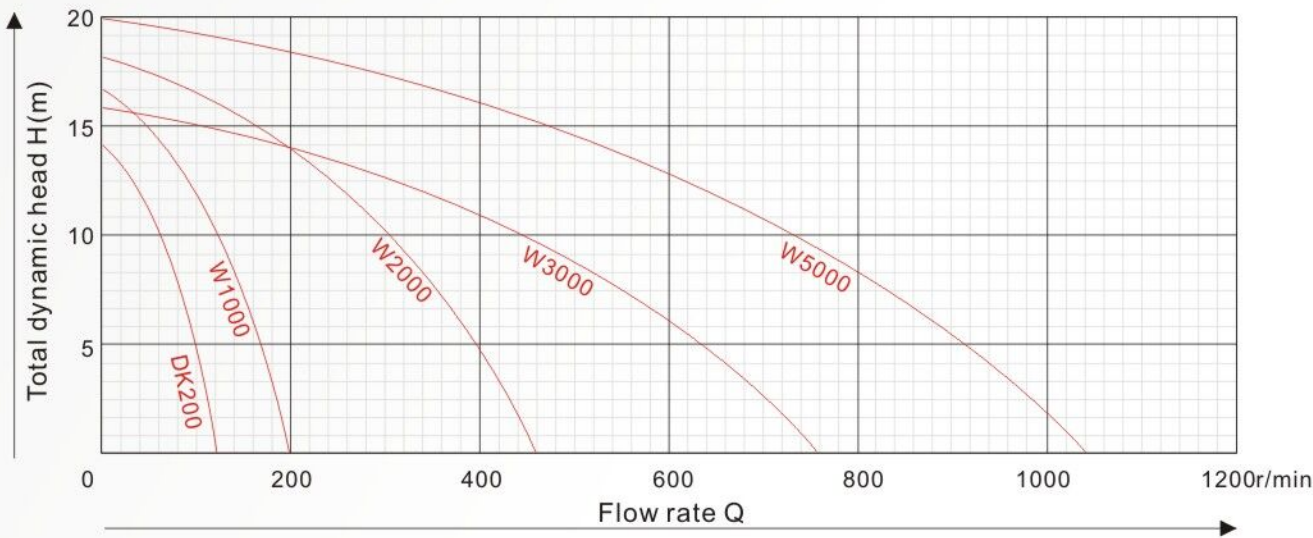
Performance chart at n=2850r/min
